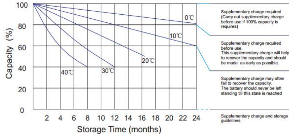
Storage characteristic
