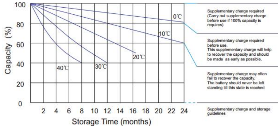
Storage characteristic
